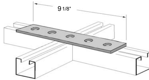
Five-Hole Splice Plate
