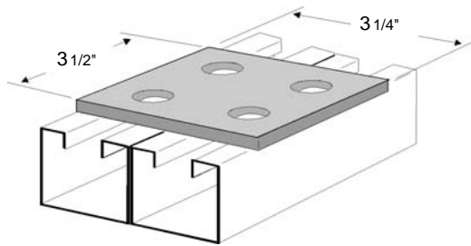
Four-Hole Splice Plate
