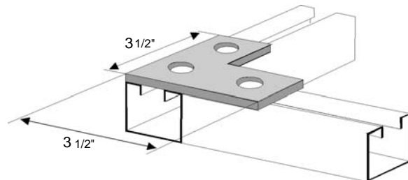
Three-Hole Corner Plate
